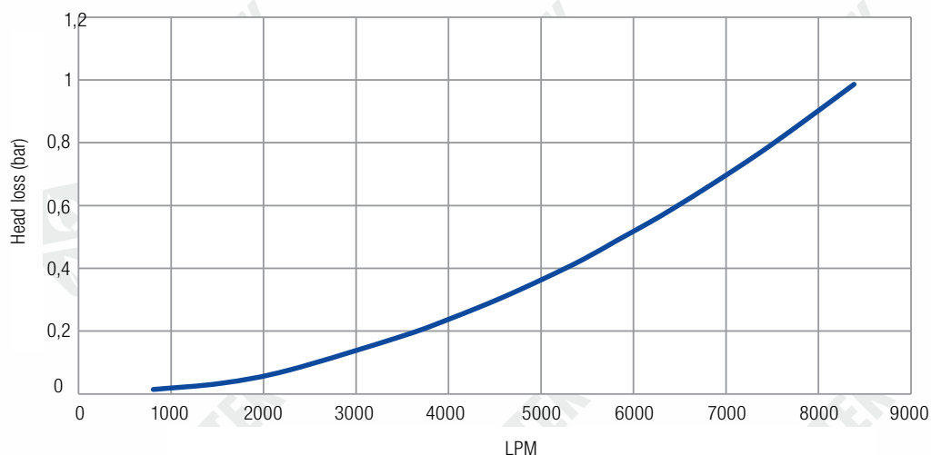
Series 27 head loss - 4.5" Pumper nozzle
